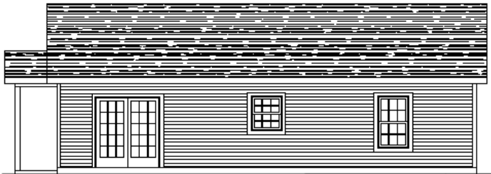
○ RIGHT ELEVATION
