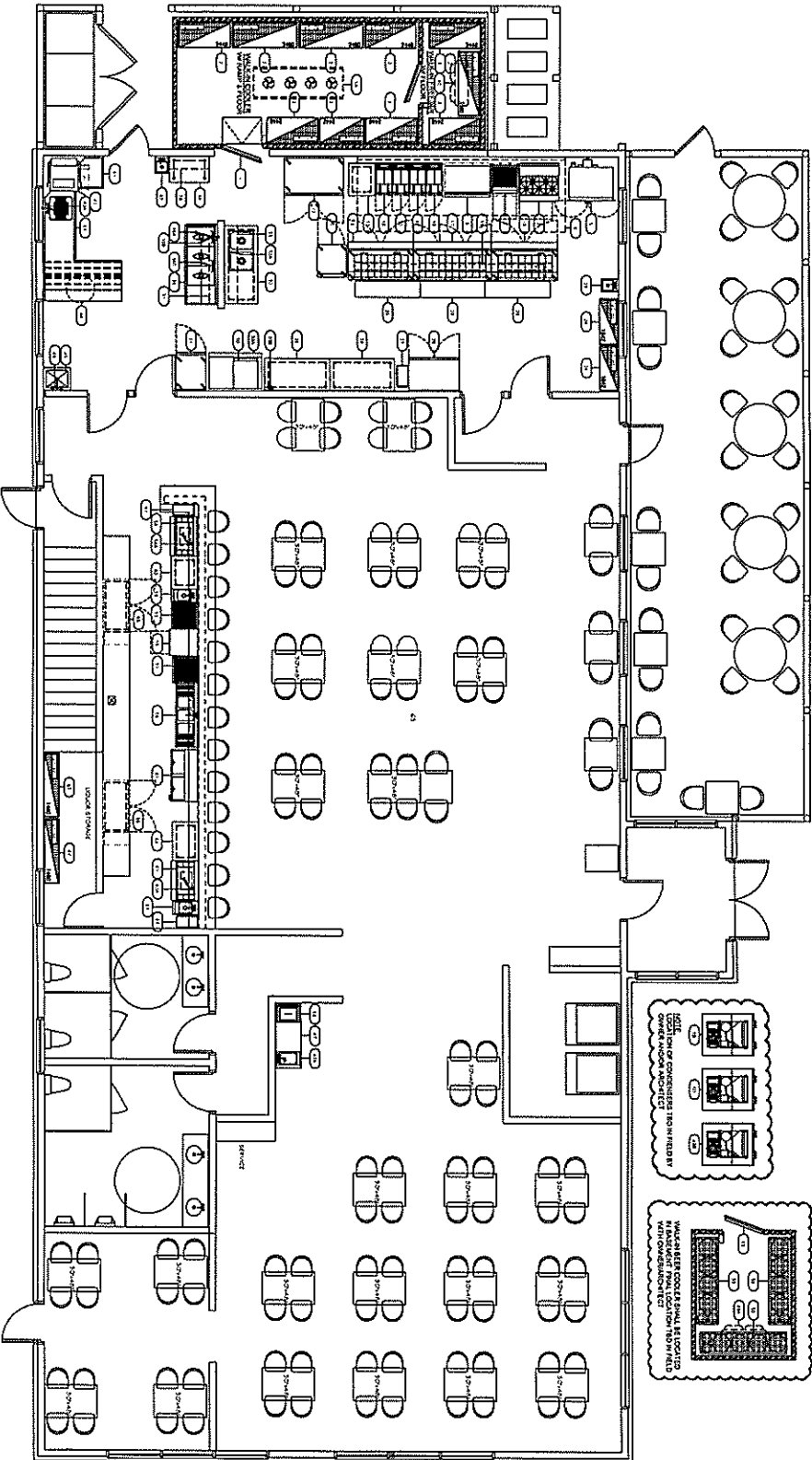
FOODSERVICE EQUIPMENT LAYOUT SCALE: 1/4" = 1'-0"
